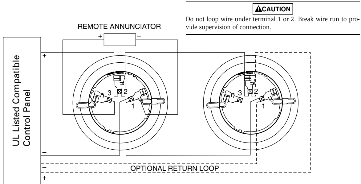
FIGURE 1. WIRING DIAGRAM:
