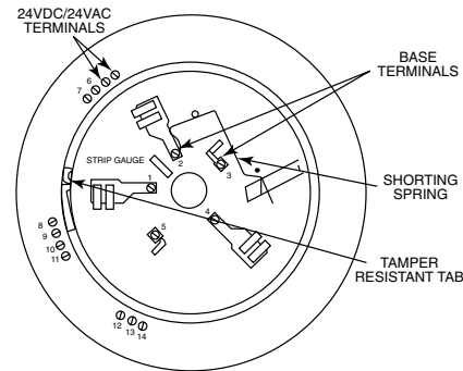
FIGURE 1. BASE TERMINALS:
