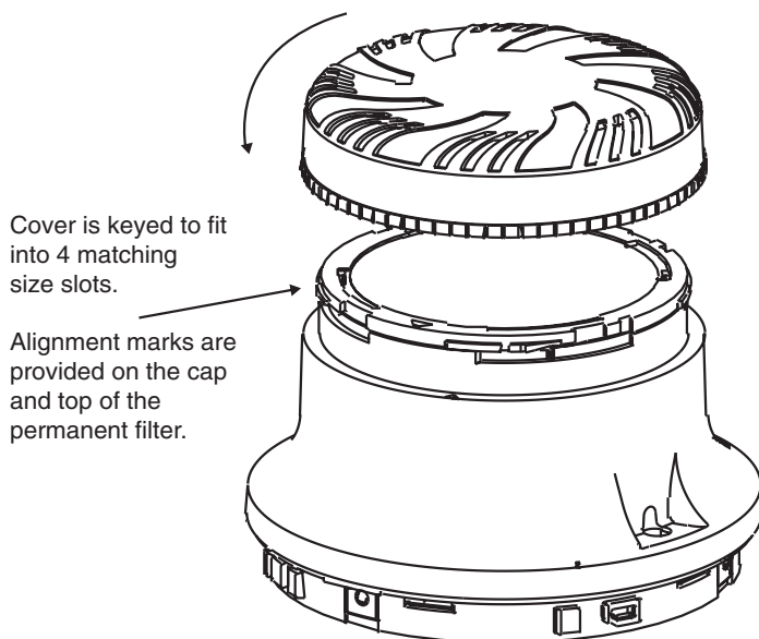
Figure 4. Replacing the filter cover:
