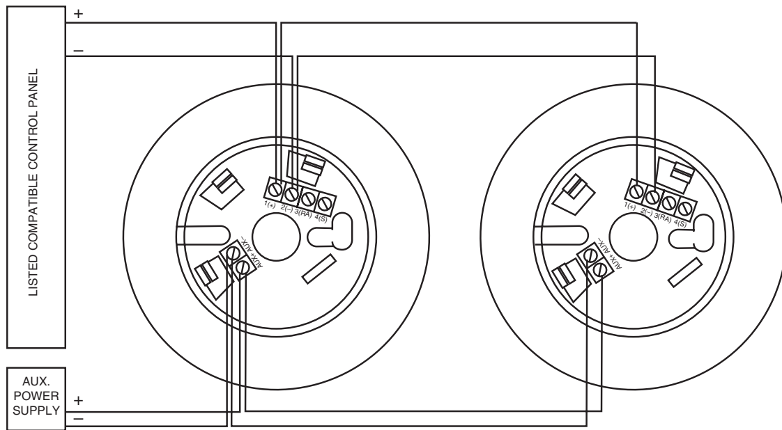
Figure 1. Wiring diagram:
