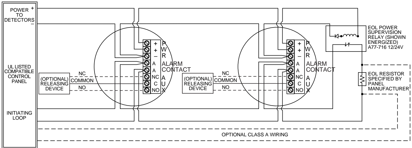
Figure 1. Wiring diagram for the 2112/24R and 2112/24TR detector:
