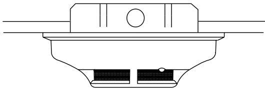
Figure 2. Surface mounting of 2112/24R and 2112/24TR smoke detector on 3½-inch and 4-inch octagonal box:
