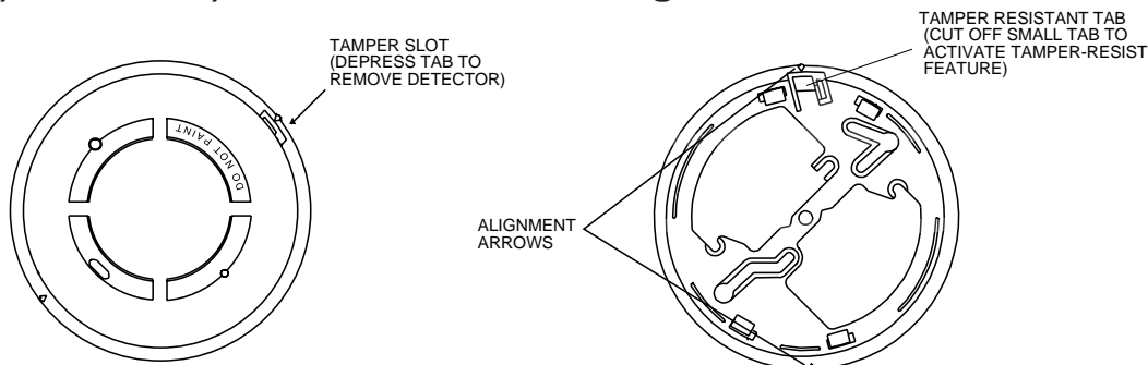
Figure 3. 2112/24R and 2112/24TR smoke detector mounting bracket:
