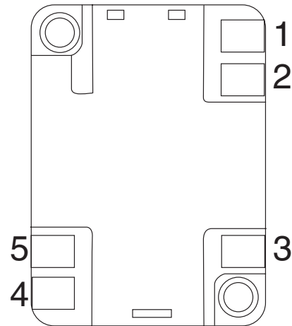
Figure 1. Terminal layout:
