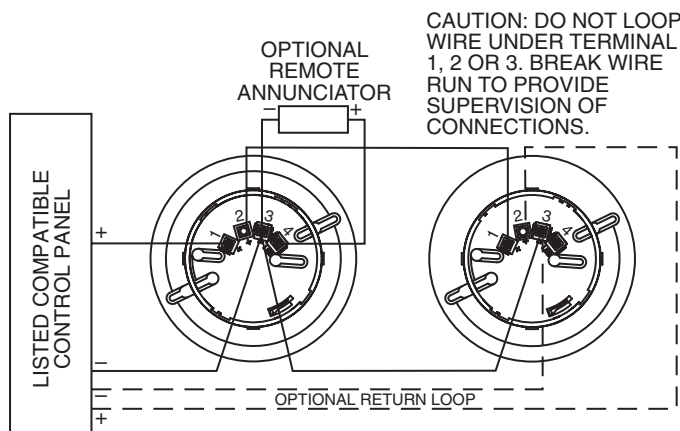
FIGURE 1. WIRING DIAGRAM:
