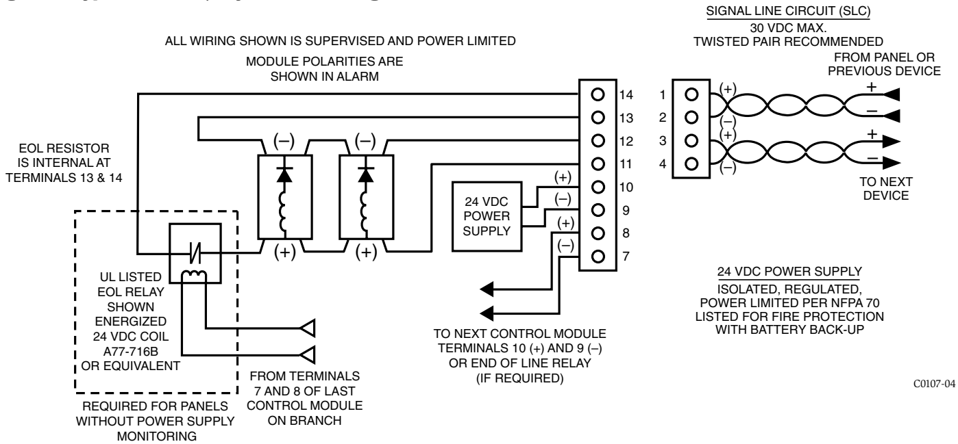
Figure 4: Typical Class B, Style Y Audio NAC configuration.
