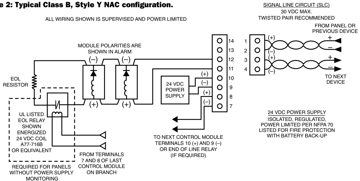
Figure 2: Typical Class B, Style Y NAC configuration.
