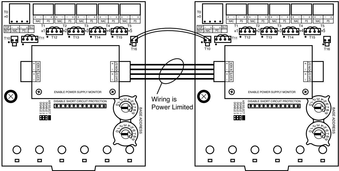
FIGURE 2: CONNECTING TWO SYNC-1 CARDS (CLASS B OPERATION, ONE POWER SUPPLY USED)
