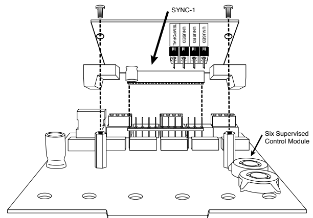
FIGURE 1: INSTALLATION OF SYNC-1
