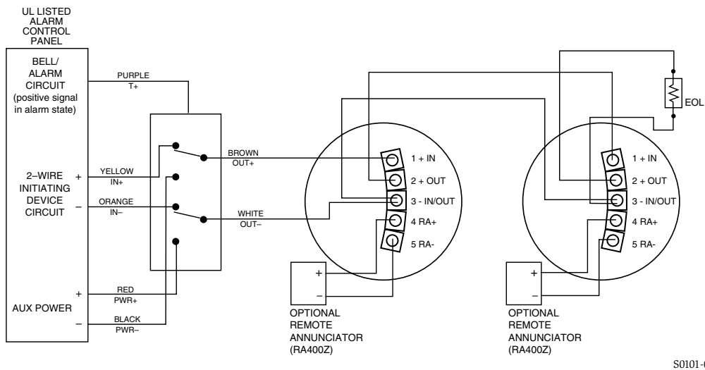
Figure 2. 4-Wire system triggered from alarm/bell output:
