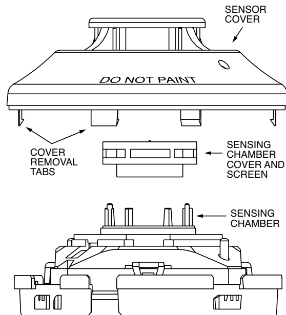
FIGURE 4. SENSOR ASSEMBLY:
